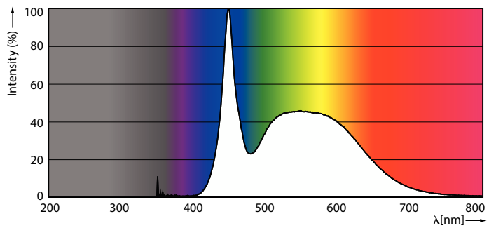
Spectral Power Distribution Colour - LEDBright 20W E27 6500K HV 1PF/12 AR
