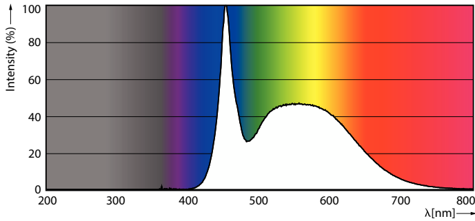
Spectral Power Distribution Colour - TForce Core HB 30W E27 865 WV G3
