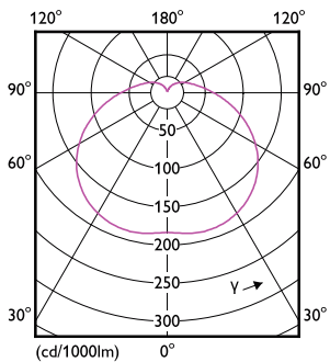
Light Distribution Diagram - TForce Core HB 30W E27 865 WV G3
